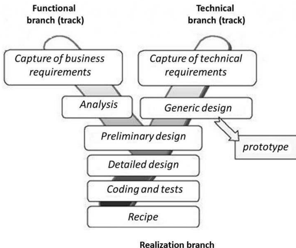
Figure 5 Two Track -unified process
