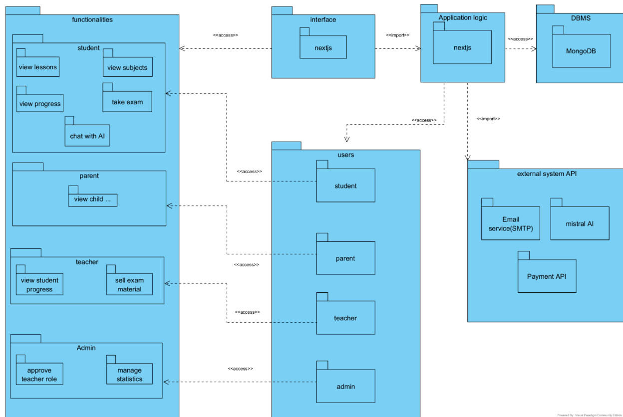
Figure 30: System Package Diagram
