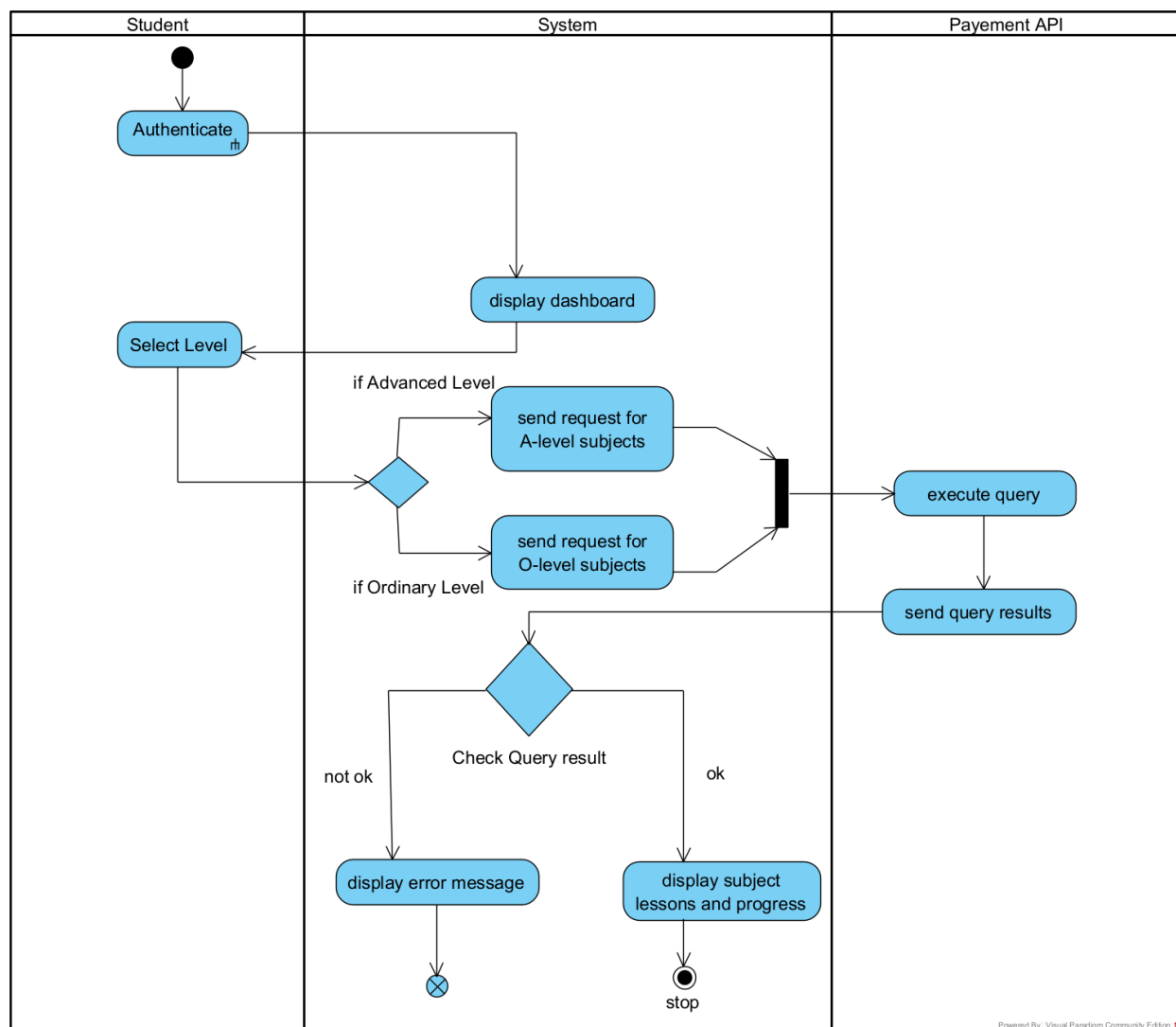
Figure 20: Level Selection Activity Diagram
