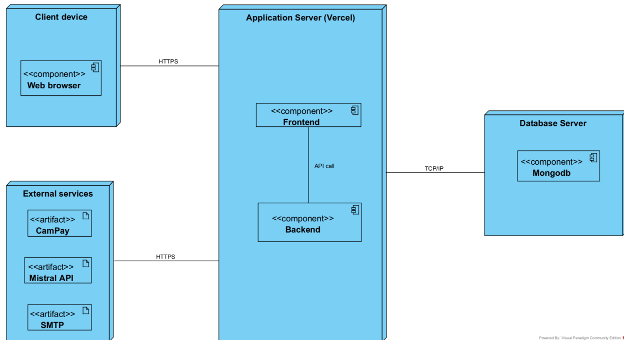
Figure 32: System Deployment Diagram
