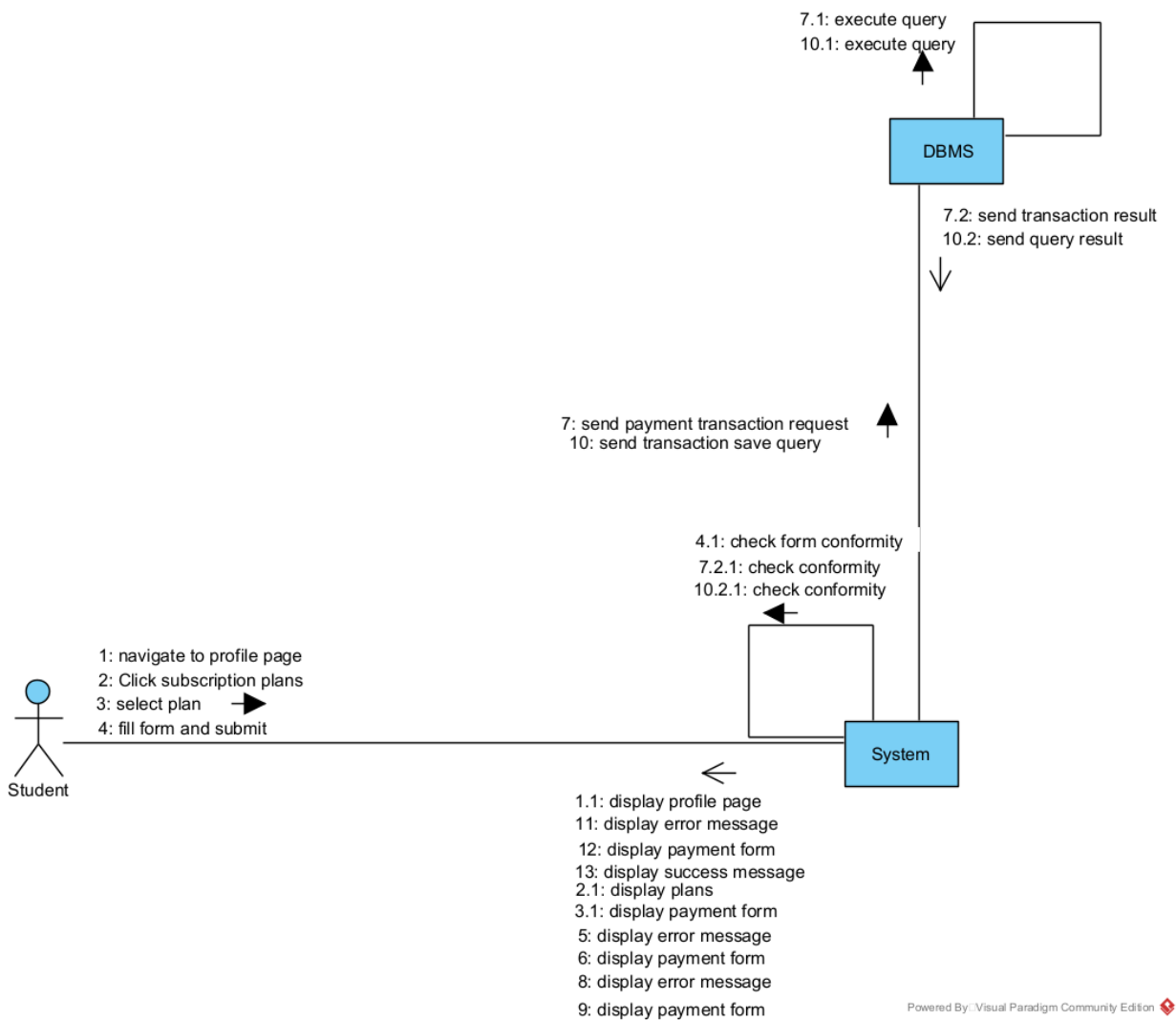
Figure 13: Make Payment Communication Diagram
