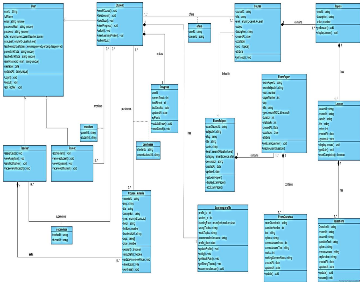
Figure 25: System Class Diagram
