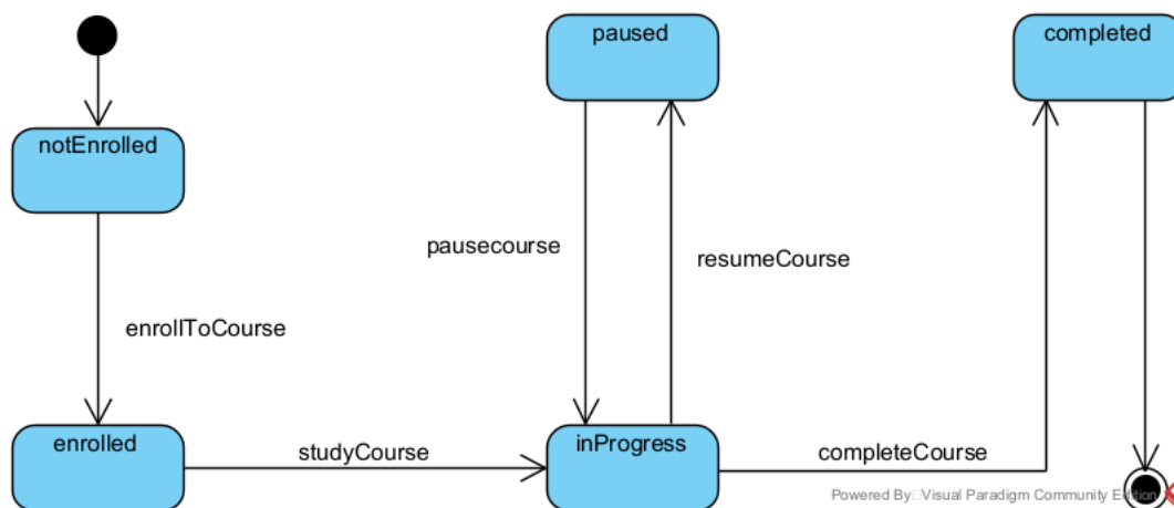
Figure 28: Student Course(Subject) State Machine Diagram
