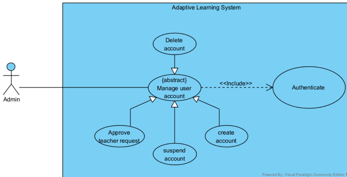
Figure 8: Manage user account
