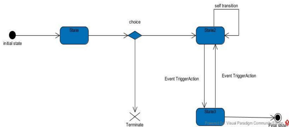
Figure 26: Formalism of the state machine diagram
