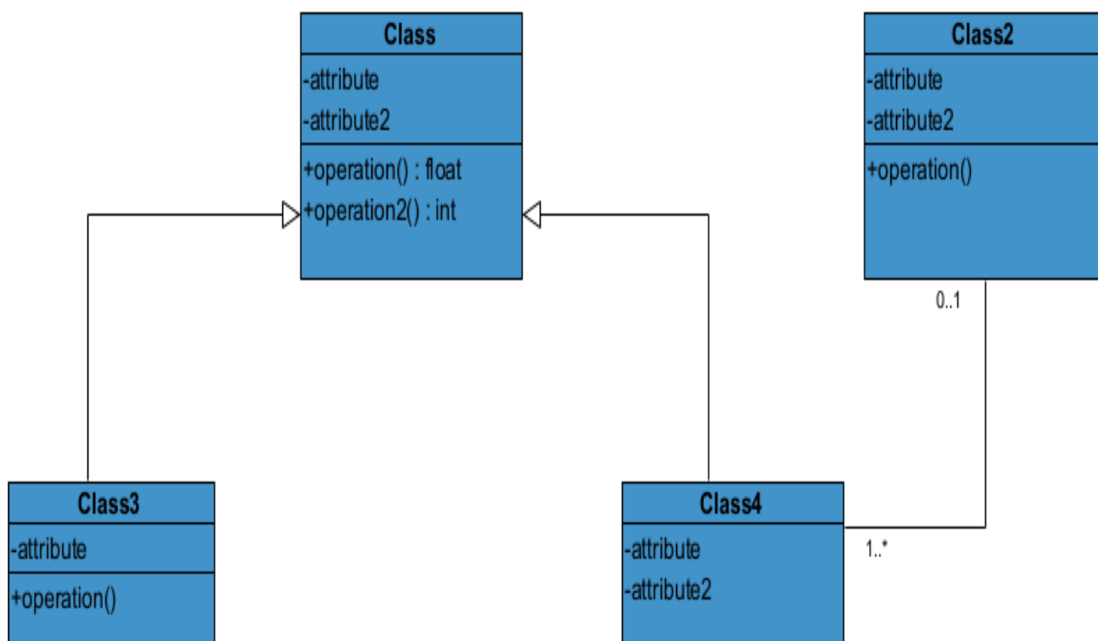
Figure 24 : formalism of class diagram
