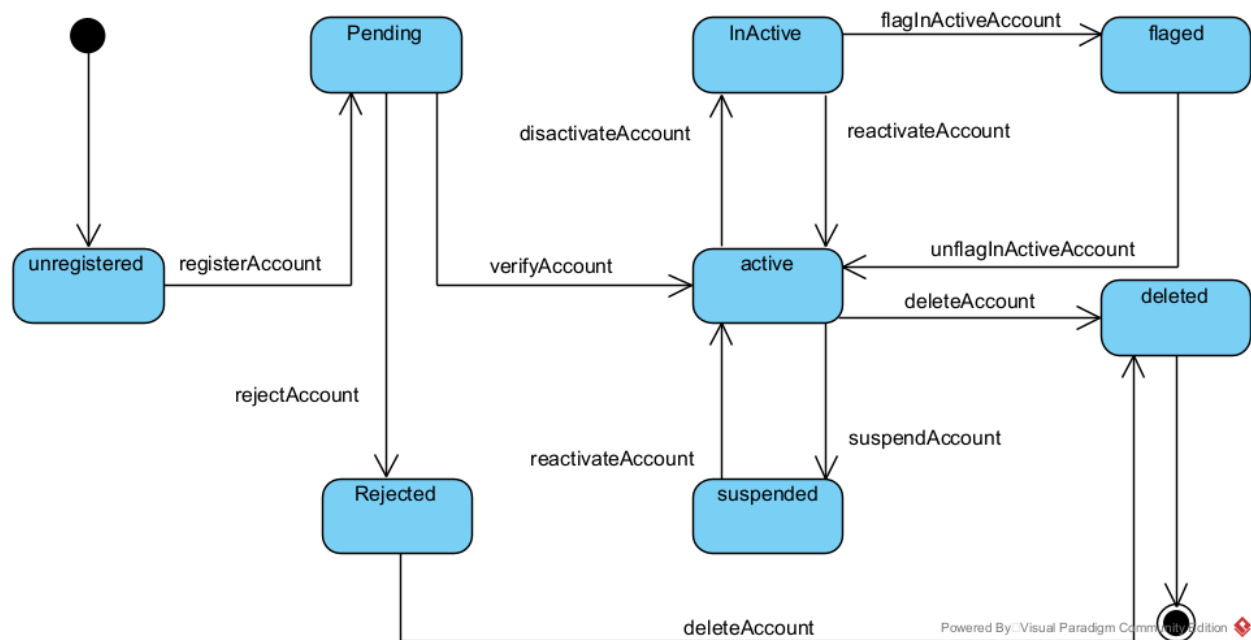
Figure 27: User State Machine Diagram
