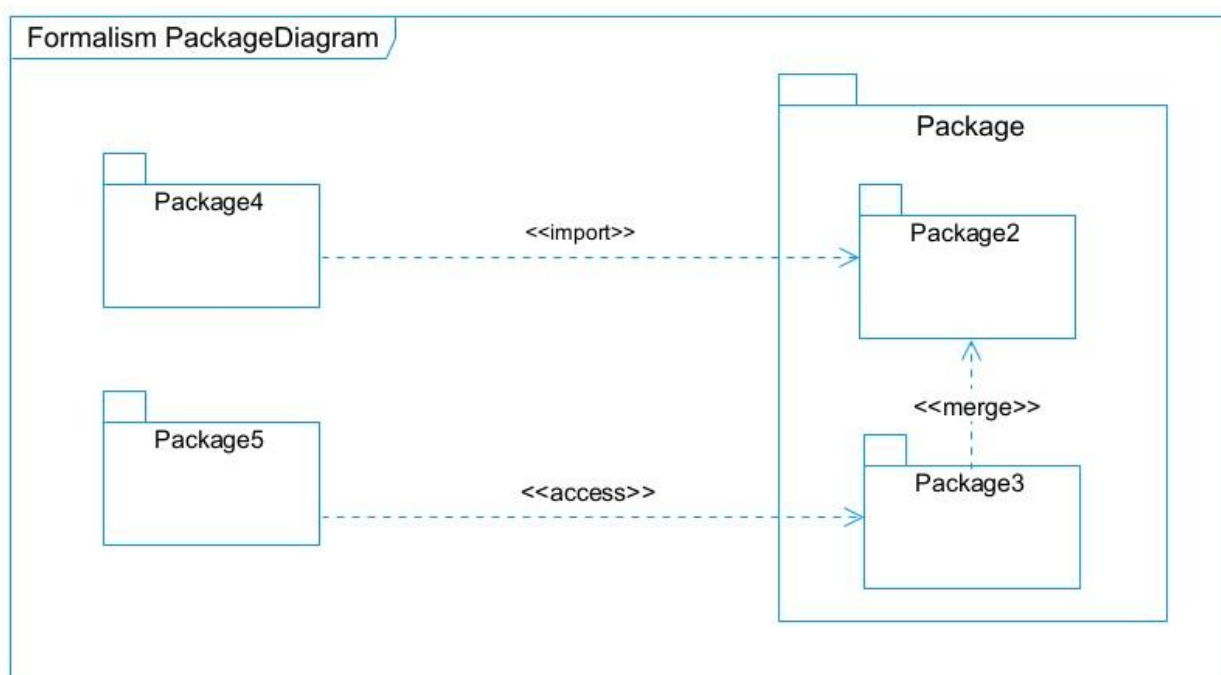
Figure 29: formalism of package diagram
