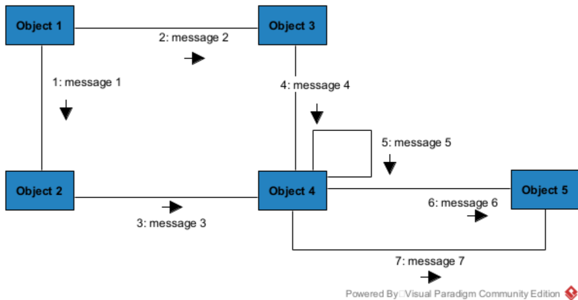
Figure 10: formalism for communication diagram
