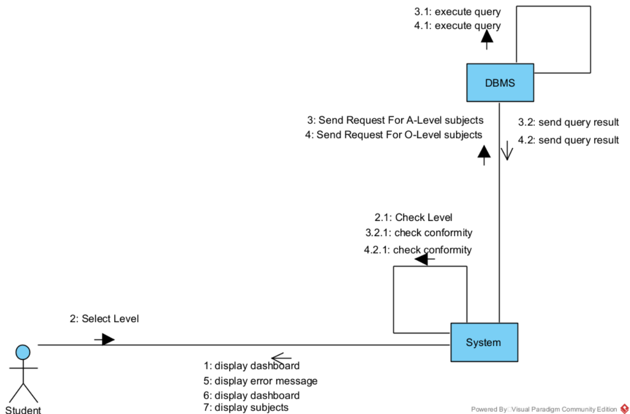
Figure 12: Select level communication diagram
