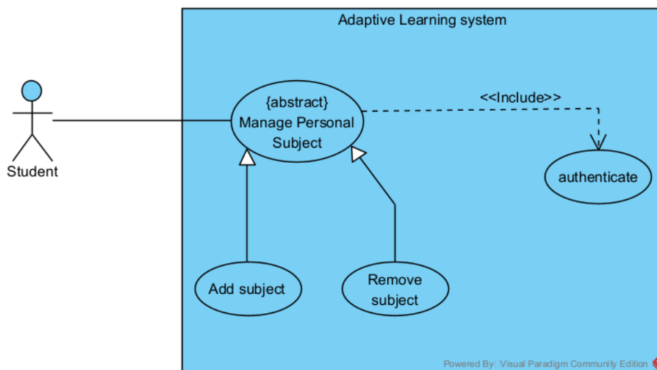
Figure 9: Manage personal subject
